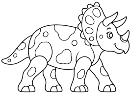
Triceratops
